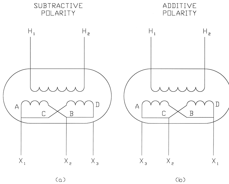
Figure 7—Single-phase transformer terminal markings (two-wire multiple connection)
